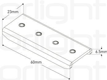
Mechanical linear Connectors x 2
