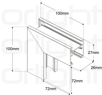
Slim Vertical 'L' Shape Connector
