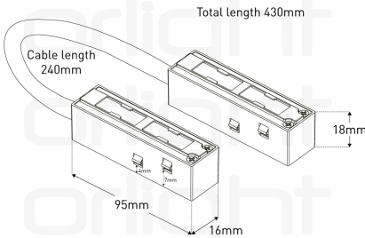
Flexible Continuous Connector
