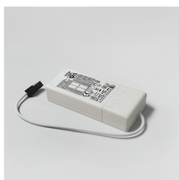
MAXDR-MINI-140MA 22247 Mini 1-10V/DALI & Push Dimming Driver
