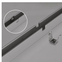
LF-SIDE-HS-SL-1M 11563 Self Locking Side Mounting Profile
