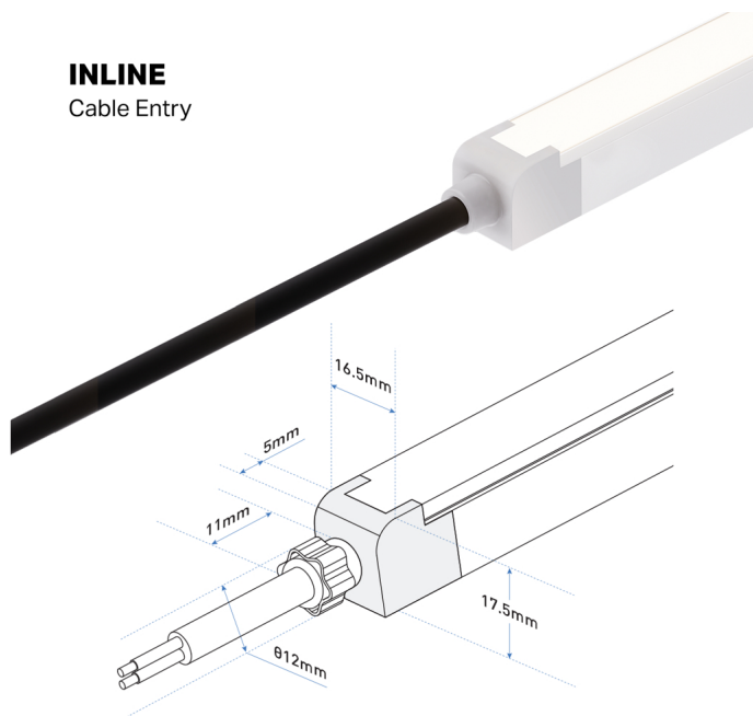
RIGHT / LEFT Cable Entry
