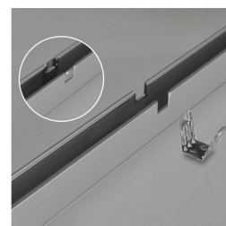
LF-SIDE-HS-SL-2M 11564 Self Locking Side Mounting Profile
