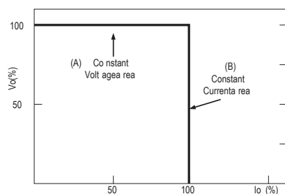
Typical LED power supply I-V curve
