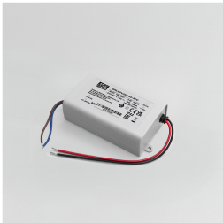
ORLRPV350-35-APC 15230 Constant current 350mA Driver
