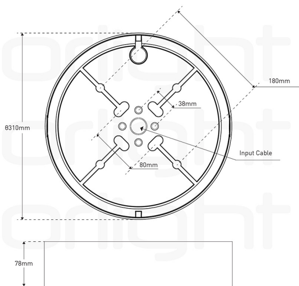
Gear Tray Fixing Details
