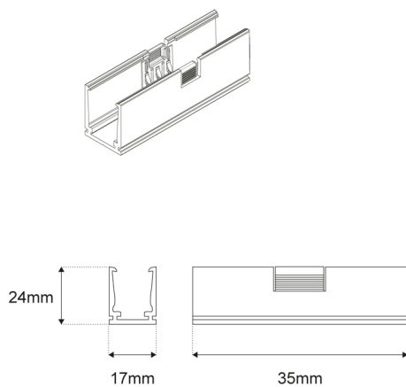
11628 - LF-TOP-HS-SL-BRACKET Self-Locking Aluminium U Channel 35mm
