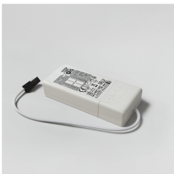
MAXDR-MINI-350MA 22251 Mini 1-10V/DALI & Push Dimming Driver
