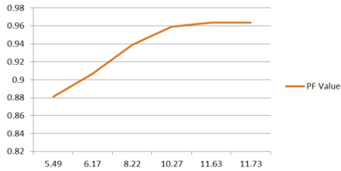
Typical Power Factor Vs Load
