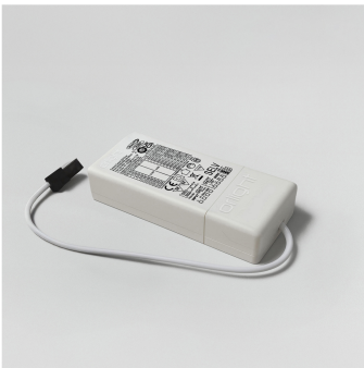
MAXDR-MINI-180MA 22248 Mini 1-10V/DALI & Push Dimming Driver
